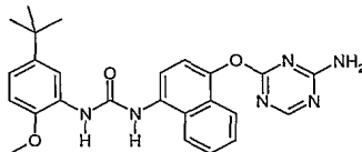
1-[4-(4-Amino-[1,3,5]triazin-2-yloxy)-naphthalen-1-yl]-3-(5-tert-butyl-2-methoxy-phenyl)-urea;
